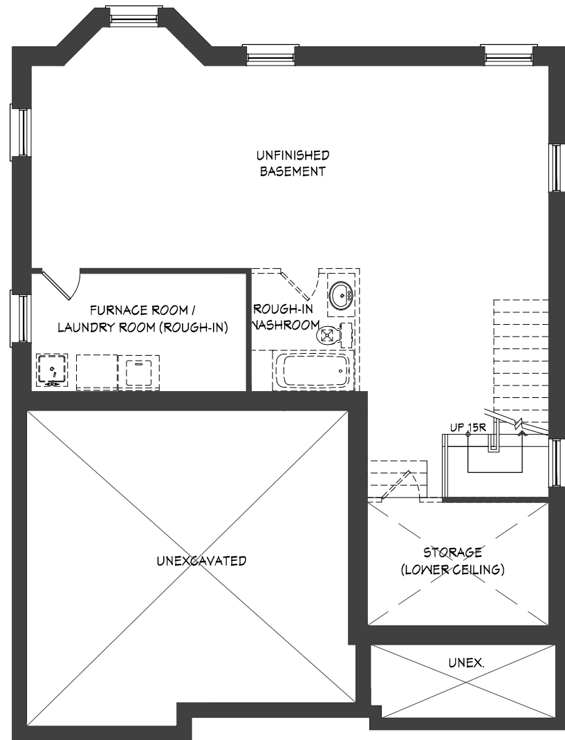
BASEMENT PLAN
