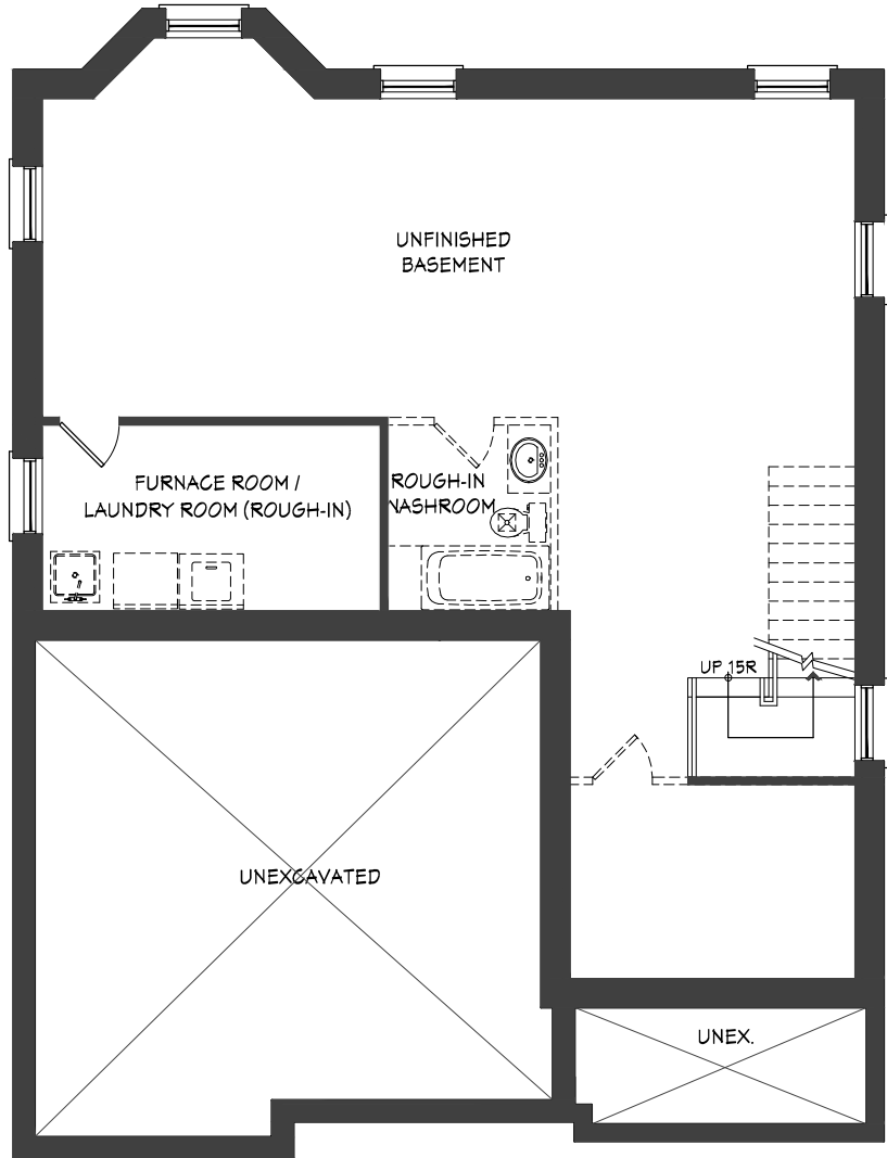
BASEMENT PLAN
