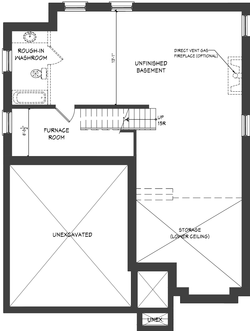
BASEMENT PLAN
