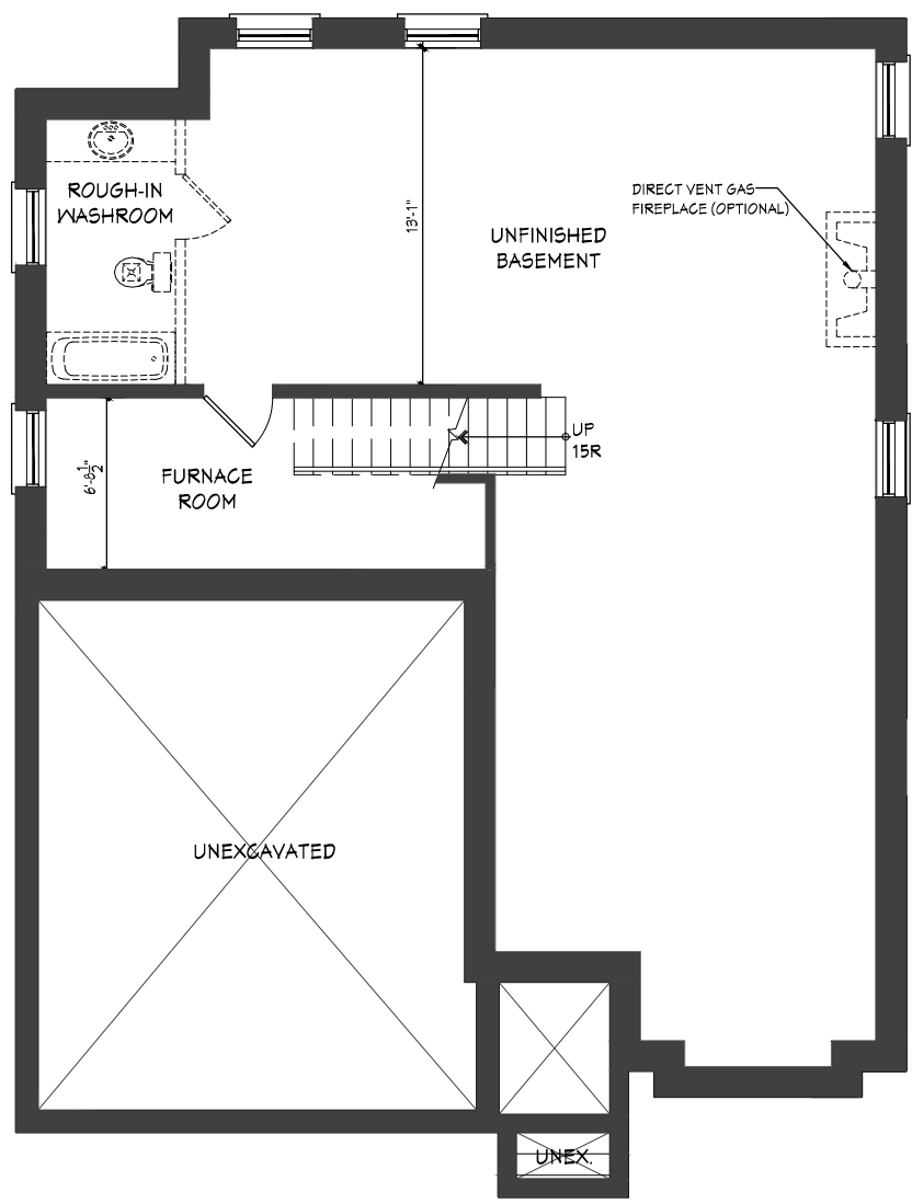
BASEMENT PLAN
