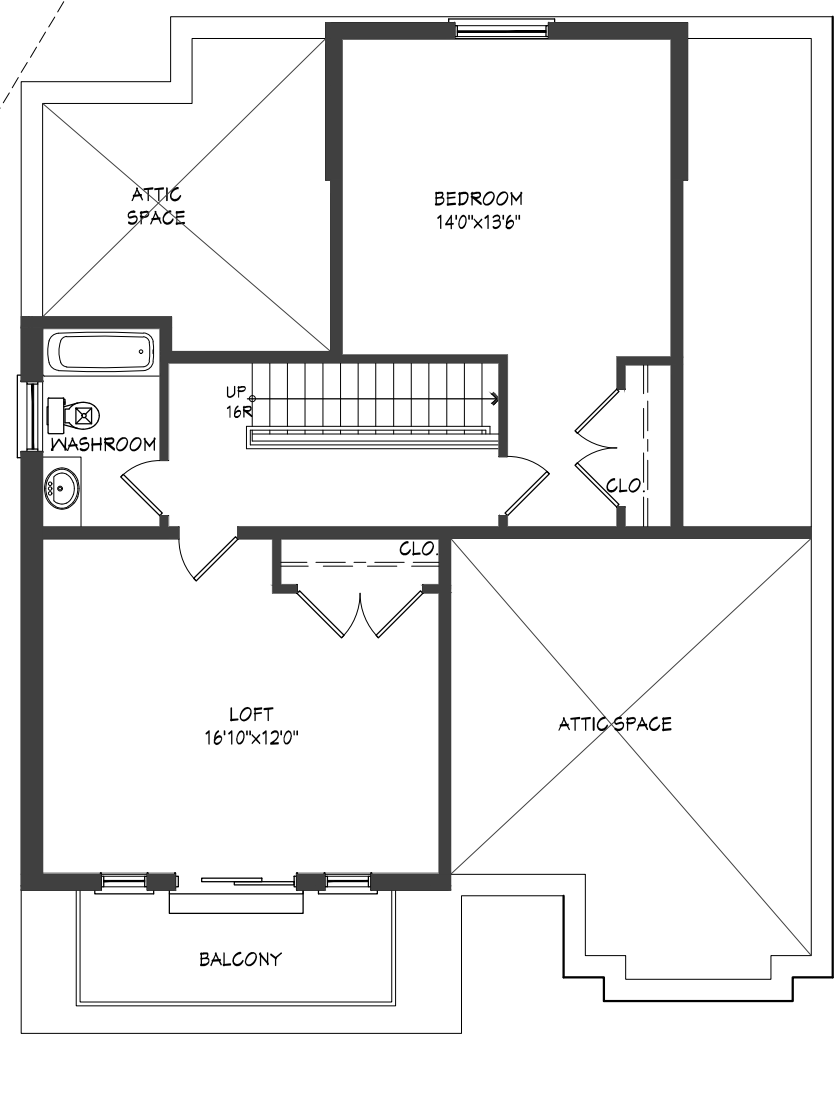
LOFT FLOOR PLAN
